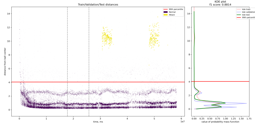
Fig. 1: Tuesday working hours. Illustration of TGN-SVDD performance. Left: On the y-axis, the anomaly score is depicted as it described in the model description. The two vertical lines imply the separation between training, validation and testing data. The red line shows the 99th percentile from the train set as a threshold. Right: Density estimation.
