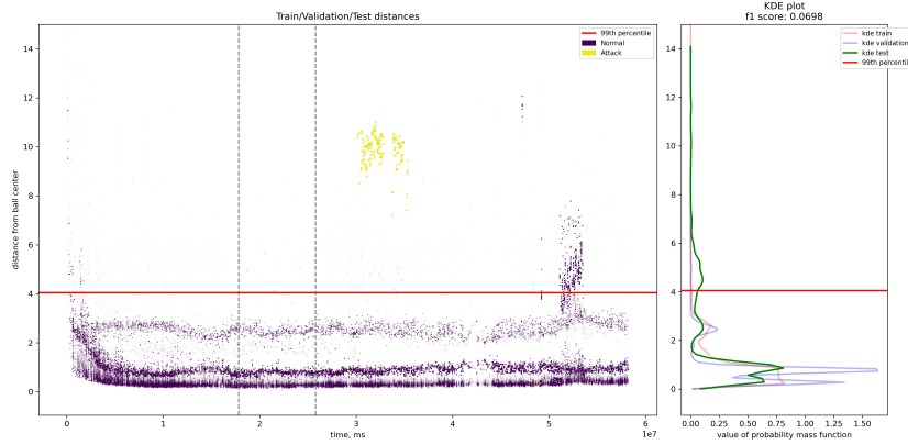
Fig. 2: Thursday working hours. Illustration of TGN-SVDD performance. Left: On the y-axis, the anomaly score is depicted as it described in the model description. The two vertical lines imply the separation between training, validation and testing data. The red line shows the 99th percentile from the train set as a threshold. Right: Density estimation.
